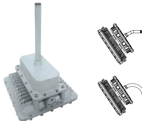
Examples using pendant mount. (Pendant pipe not included.)
